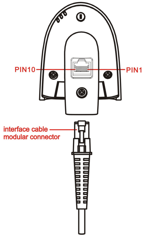
Cable connector interface pin-outs
